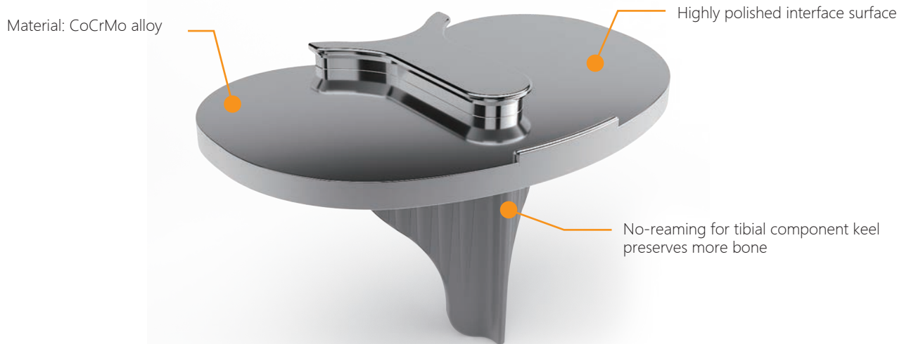
PreciTotal, Stemmed Tray, Polished
